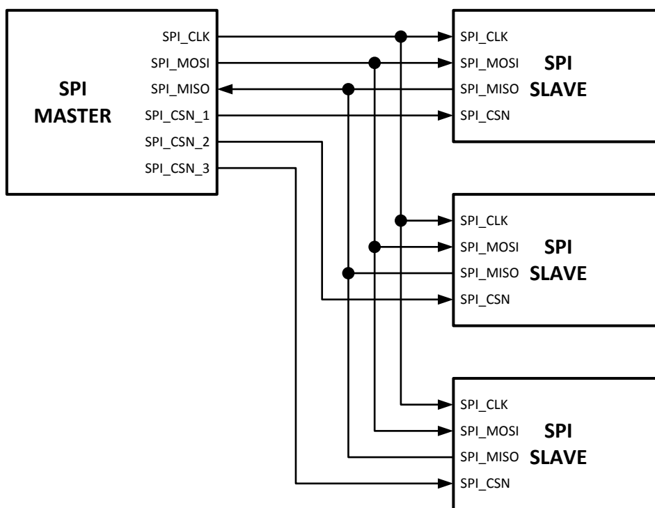
Figure 22: SPI with 1 Master and 3 Slaves
